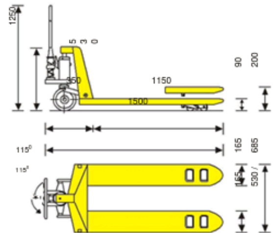
Paper Roll Lifting with Taper Fork Pallet Truck
